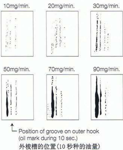
Fig.2 : Oil mark and oil amount.
